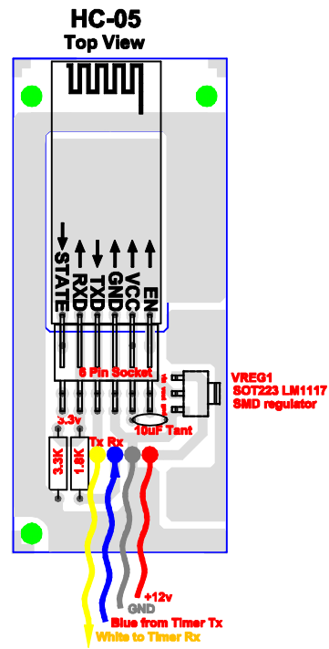
Serial to Bluetooth using IOIO mounts
